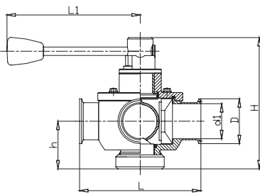
3-Wege Bogenventil Serie 21, manuell, TC-Clamp 3-way arc valve series 21, manual, TC-clamp
