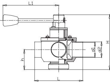
3-Wege Bogenventil Serie 21, manuell, Schweißende 3-way arc valve series 21, manual, welded ends
